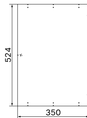
16-Lower drawer front panel
