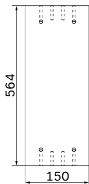
4-Stiffening rib
