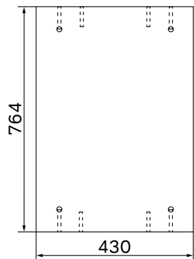
3-Bottom panel
