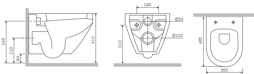
FlashClean C701700WH
